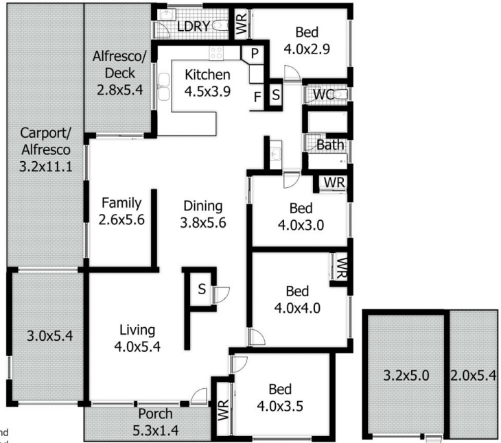
FLOOR PLAN
